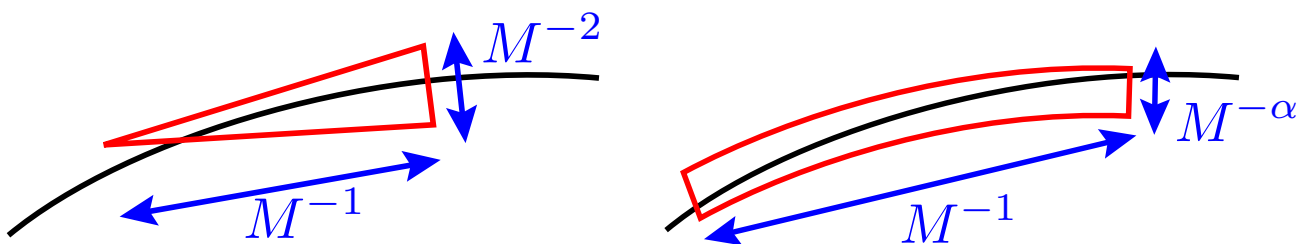
Fig. 9.6. A Wavelet Tour of Signal Processing, 3 rd ed. Adapted triangle and finite element to approximate a discontinuous function around a singularity curve.
