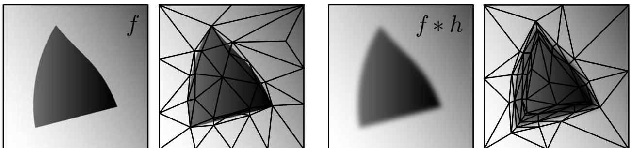
Fig. 9.5. A Wavelet Tour of Signal Processing, 3 rd ed. Adaptive triangulations for piecewise linear approximations of a piecewise C^2 image, without and with a blurring kernel.
