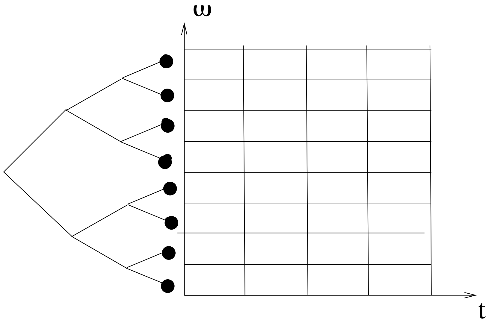
Fig. 8.9. A Wavelet Tour of Signal Processing, 3 rd ed. Admissible tree and Heisenberg boxes of a wavelet packet pseudo local cosine basis.
