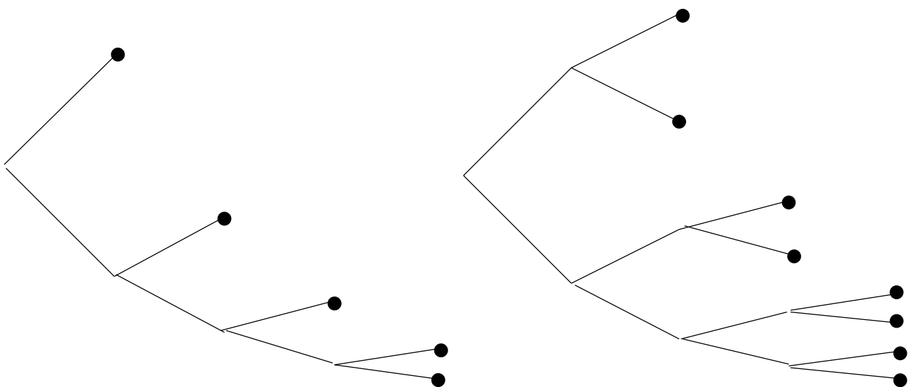
Fig. 8.7. A Wavelet Tour of Signal Processing, 3 rd ed. (a): Wavelet packet tree of a dyadic wavelet basis. (b): Wavelet packet tree of an M-band wavelet basis with M = 2 .
