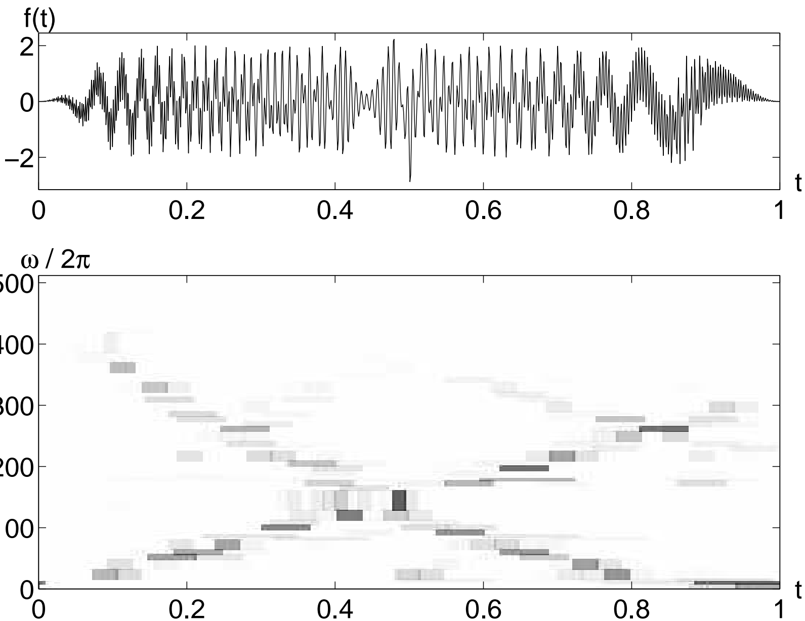
Fig. 8.6. A Wavelet Tour of Signal Processing, 3 rd ed. Wavelet packet decomposition of the multi-chirp signal. The darker the gray level of each Heisenberg box the larger the amplitude |\langle f, \psi_j^p \rangle| of the corresponding wavelet packet coefficient.
