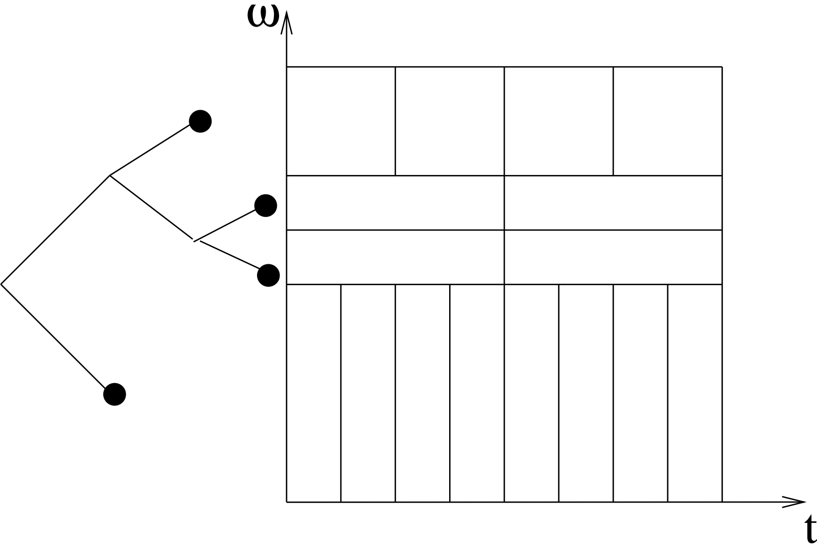
Fig. 8.5. A Wavelet Tour of Signal Processing, 3 rd ed. The wavelet packet tree on the left divides the frequency axis in several intervals. The Heisenberg boxes of the corresponding wavelet packet basis are on the right.
