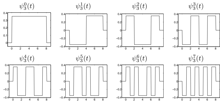
Fig. 8.4. A Wavelet Tour of Signal Processing, 3 rd ed. Frequency ordered Walsh wavelet packets computed with a Haar filter, at the depth j - L = 3 of the wavelet packet tree, with L = 0 .
