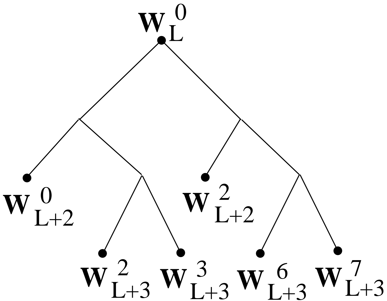
Fig. 8.3. A Wavelet Tour of Signal Processing, 3 rd ed. Example of admissible wavelet packet binary tree.
