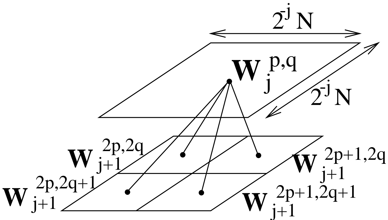
Fig. 8.21. A Wavelet Tour of Signal Processing, 3 rd ed. Functions in W_j^{p,q} have a support located in a square region of the image. It is divided into four subspaces that cover smaller squares in the image.
