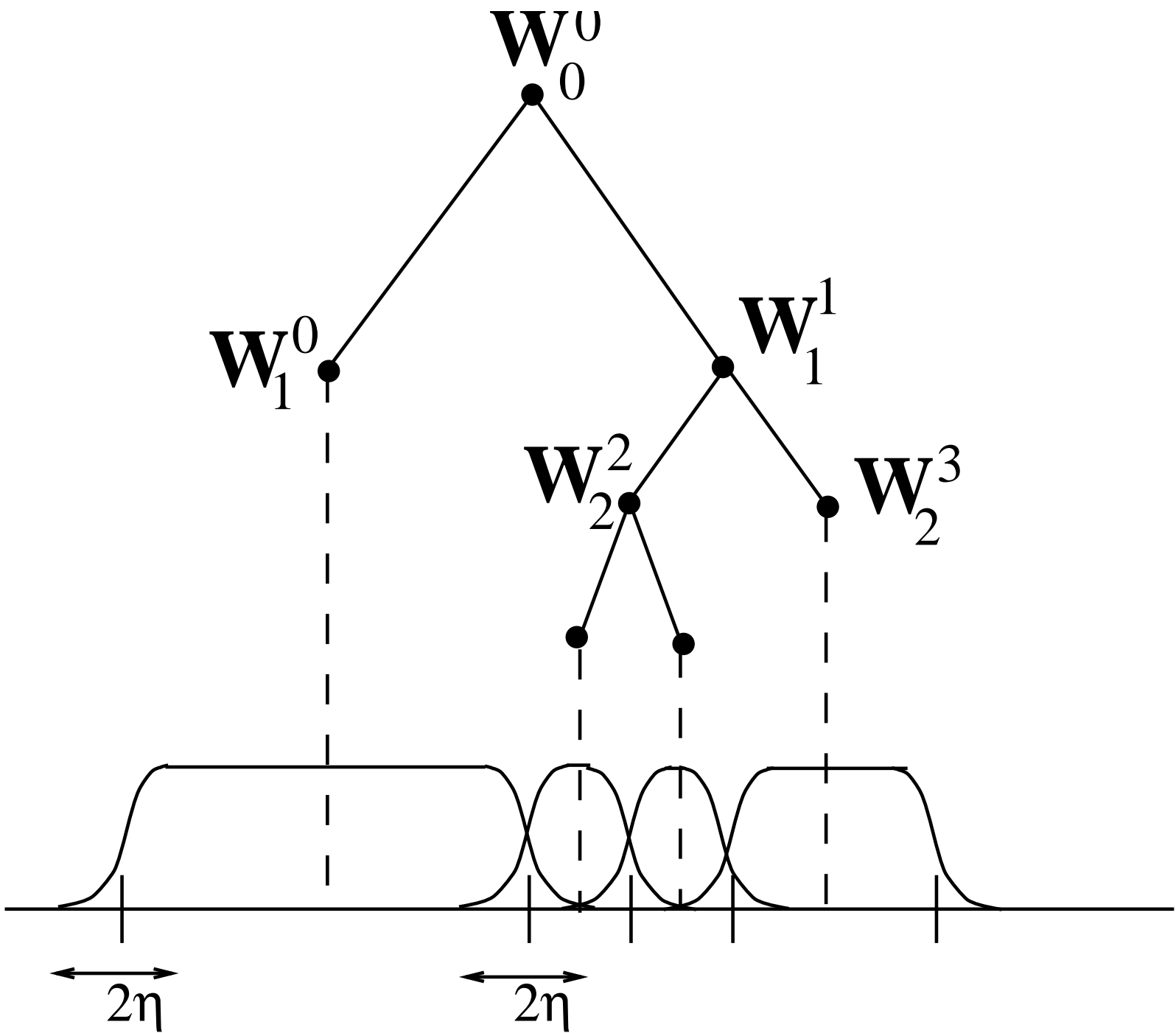
Fig. 8.20. A Wavelet Tour of Signal Processing, 3 rd ed. An admissible binary tree of local cosine spaces divides the time axis in windows of dyadic lengths.
