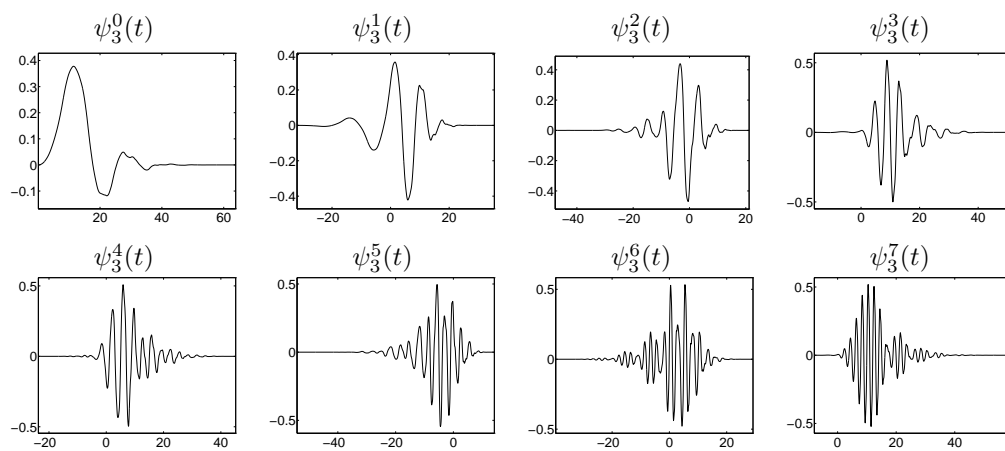
Fig. 8.2. A Wavelet Tour of Signal Processing, 3 rd ed. Wavelet packets computed with the Daubechies 5 filter, at the depth j - L = 3 of the wavelet packet tree, with L = 0 . They are ordered from low to high frequencies.
