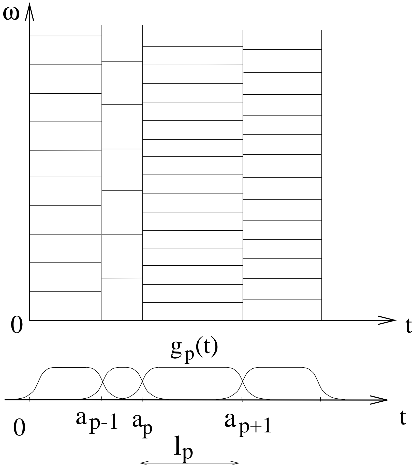
Fig. 8.18. A Wavelet Tour of Signal Processing, 3 rd ed. The Heisenberg boxes of local cosine vectors define a regular grid over the time-frequency plane.
