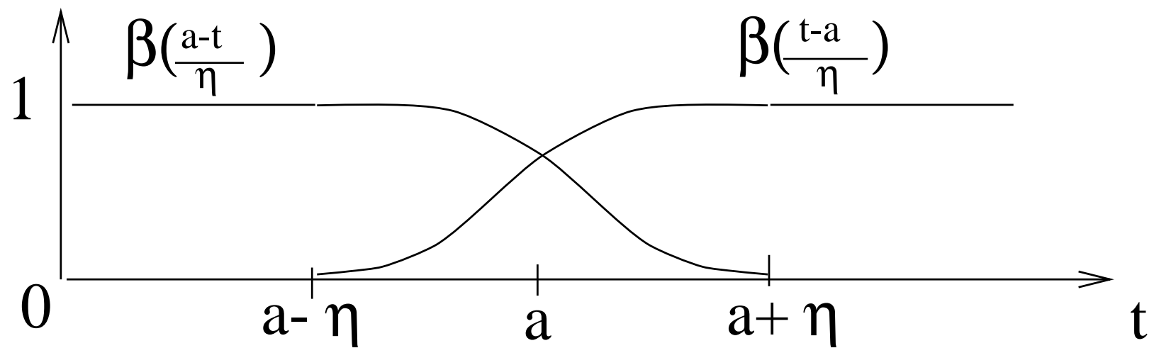
Fig. 8.16. A Wavelet Tour of Signal Processing, 3 rd ed. A multiplication with \beta\left(\frac{t-a}{\eta}\right) and \beta\left(\frac{a-t}{\eta}\right) restricts the support of functions to [a - \eta, +\infty) and (-\infty, a + \eta]
