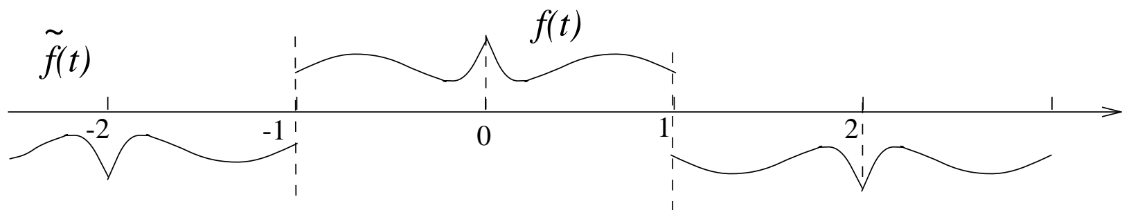
Fig. 8.15. A Wavelet Tour of Signal Processing, 3 rd ed. A cosine IV extends f(t) into a signal \tilde{f}(t) of period 4 which is symmetric with respect to 0 and antisymmetric with respect to 1.
