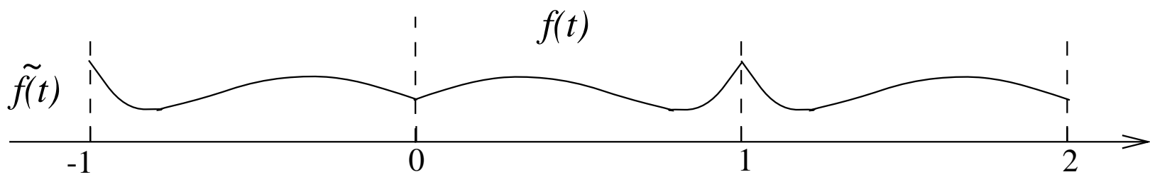
Fig. 8.14. A Wavelet Tour of Signal Processing, 3 rd ed. The function \tilde{f}(t) is an extension of f(t) ; it is symmetric about 0 and of period 2.
