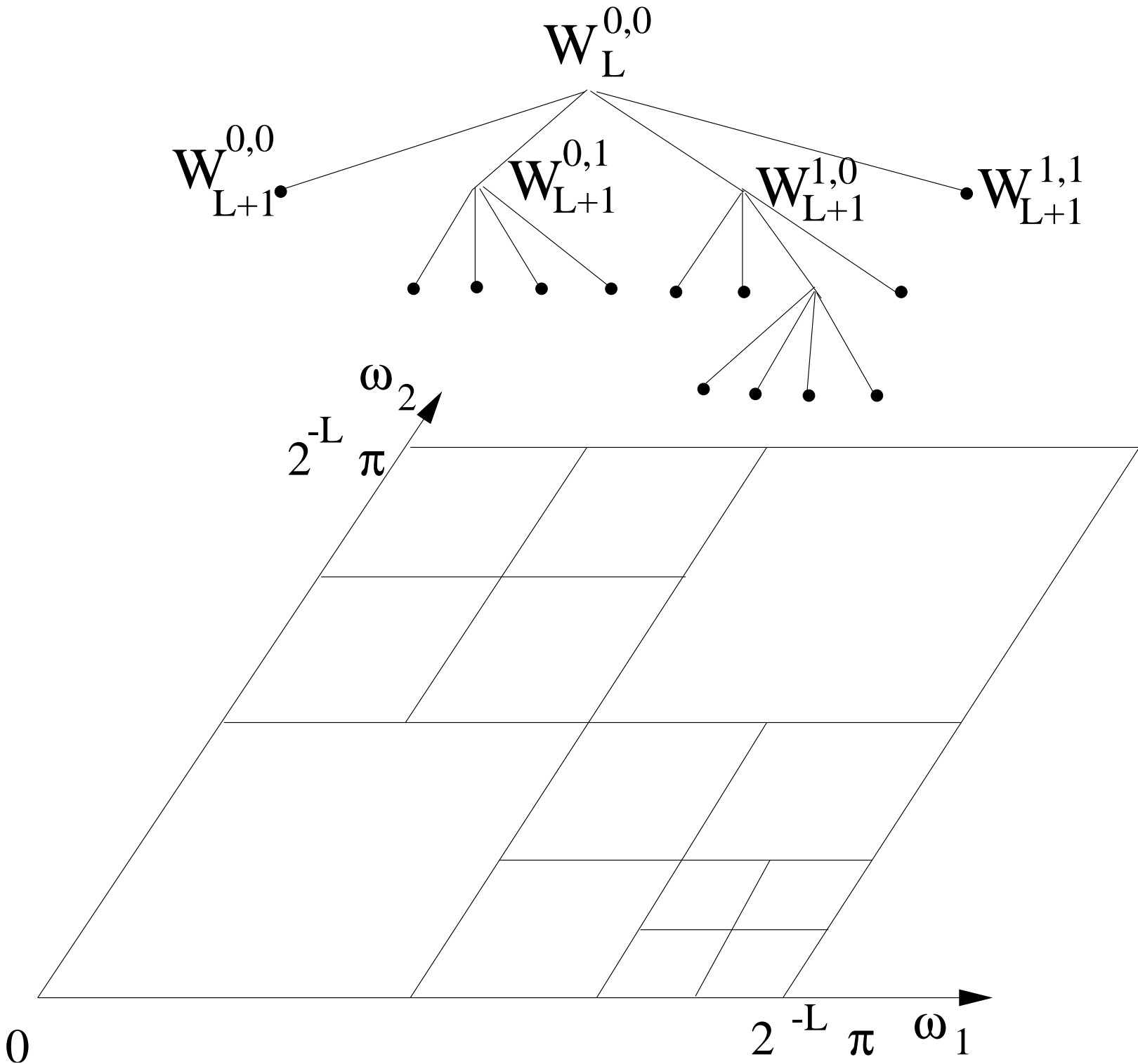
Fig. 8.12. A Wavelet Tour of Signal Processing, 3 rd ed. A wavelet packet quad-tree decomposes the positive frequency quadrant into squares of progressively smaller sizes as we go down the tree.
