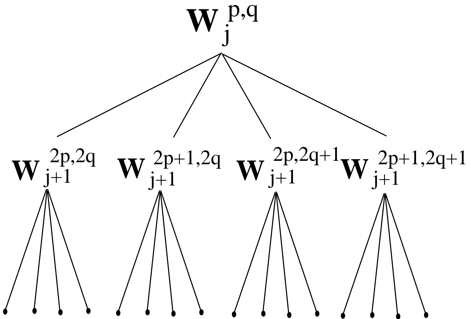
Fig. 8.11. A Wavelet Tour of Signal Processing, 3 rd ed. A wavelet packet quad-tree for images is constructed recursively by decomposing each separable space \mathbf{W}_j^{p,q} in four subspaces.
