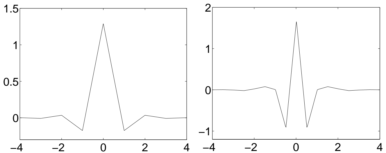
Fig. 7.9. A Wavelet Tour of Signal Processing, 3 rd ed. Linear spline Battle-Lemarié scaling function \phi and wavelet \psi .
