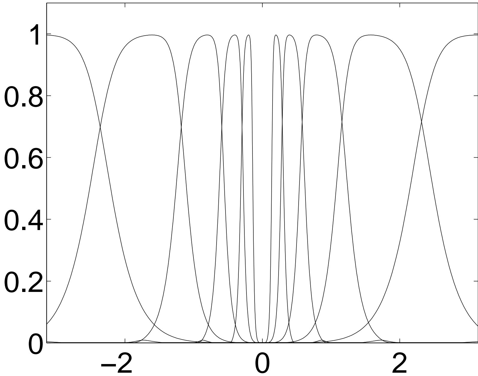
Fig. 7.6. A Wavelet Tour of Signal Processing, 3 rd ed. Graphs of |\hat{\psi}(2^j \omega)|^2 for the cubic spline Battle-Lemarié wavelet, with 1 \leq j \leq 5 and \omega \in [-\pi, \pi] .
