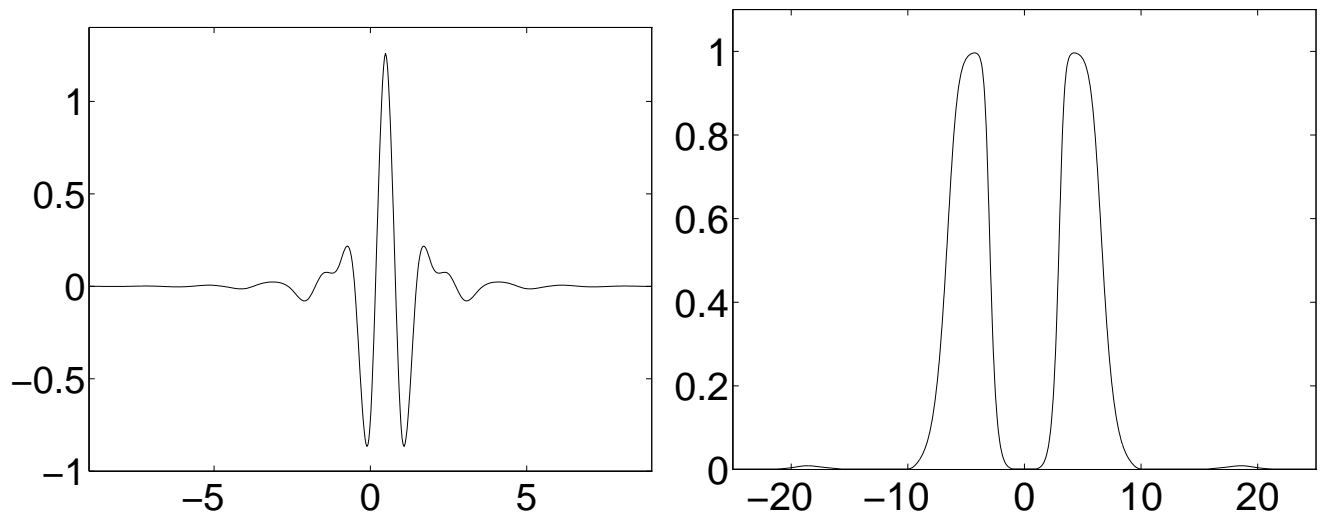
Fig. 7.5. A Wavelet Tour of Signal Processing, 3 rd ed. Battle-Lemarié cubic spline wavelet \psi and its Fourier transform modulus.
