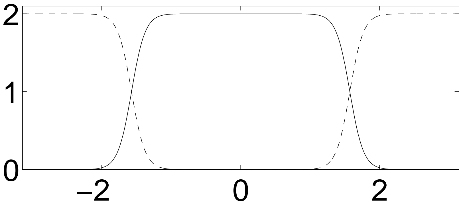
Fig. 7.4. A Wavelet Tour of Signal Processing, 3 rd ed. The solid line gives |\hat{h}(\omega)|^2 on [-\pi, \pi] , for a cubic spline multiresolution. The dotted line corresponds to |\hat{g}(\omega)|^2 .
