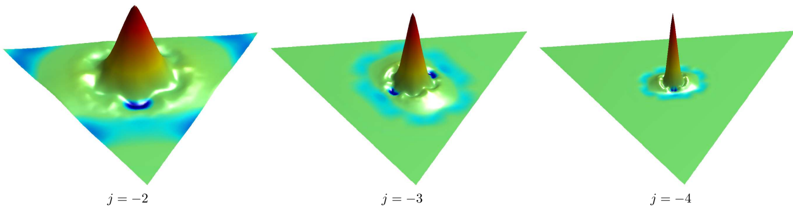
Fig. 7.35. A Wavelet Tour of Signal Processing, 3 rd ed. Example of dual wavelets \tilde{\psi}_{j,k}(x) for x on a subdivided equilateral triangle. The height over the triangle indicates the value of the wavelet.
