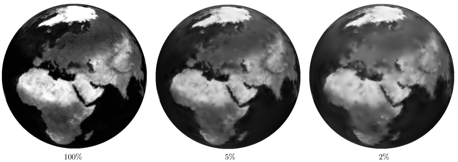
Fig. 7.34. A Wavelet Tour of Signal Processing, 3 rd ed. Non-linear approximation of a function defined on a sphere using a decreasing number of large wavelet coefficients.
