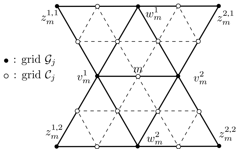
Fig. 7.33. A Wavelet Tour of Signal Processing, 3 rd ed. Labeling of points in the butterfly neighborhood of a vertex m \in \mathcal{H}_j .
