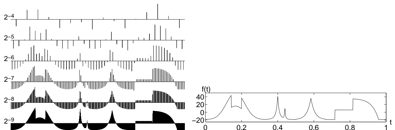
Fig. 7.3. A Wavelet Tour of Signal Processing, 3 rd ed. Discrete multiresolution approximations a_j[n] at scales 2^j , computed with cubic splines.
