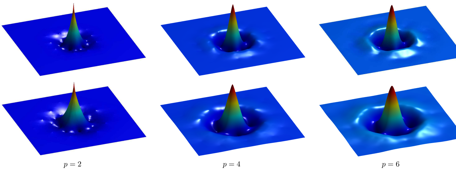
Fig. 7.29. A Wavelet Tour of Signal Processing, 3 rd ed. Quincunx dual wavelets \tilde{\psi}_{i,j,m} and \tilde{\psi}_{i,j+1,m} at two consecutive scales 2^j and 2^{j+1/2} (first and second row), with progressively more vanishing moments.
