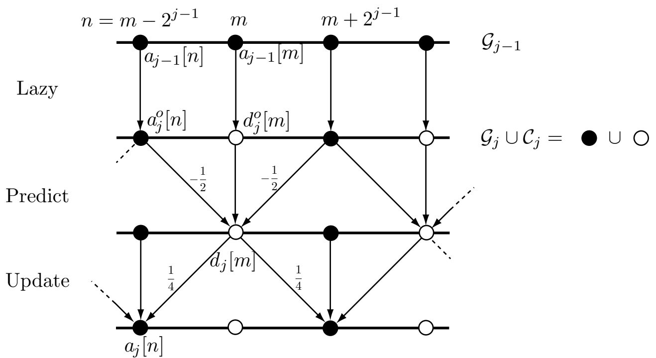
Fig. 7.27. A Wavelet Tour of Signal Processing, 3 rd ed. Predict and update steps for the construction of linear spline wavelets.
