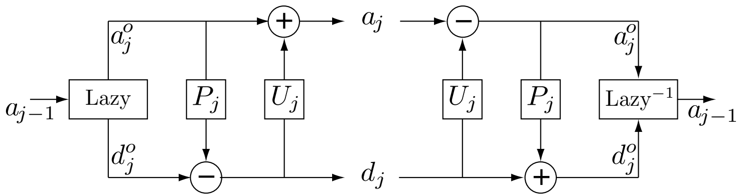
Fig. 7.26. A Wavelet Tour of Signal Processing, 3 rd ed. Predict and update decomposition of a_{j-1} into a_j and d_j , followed by the reconstruction of a_{j-1} with the same update and predict operators.
