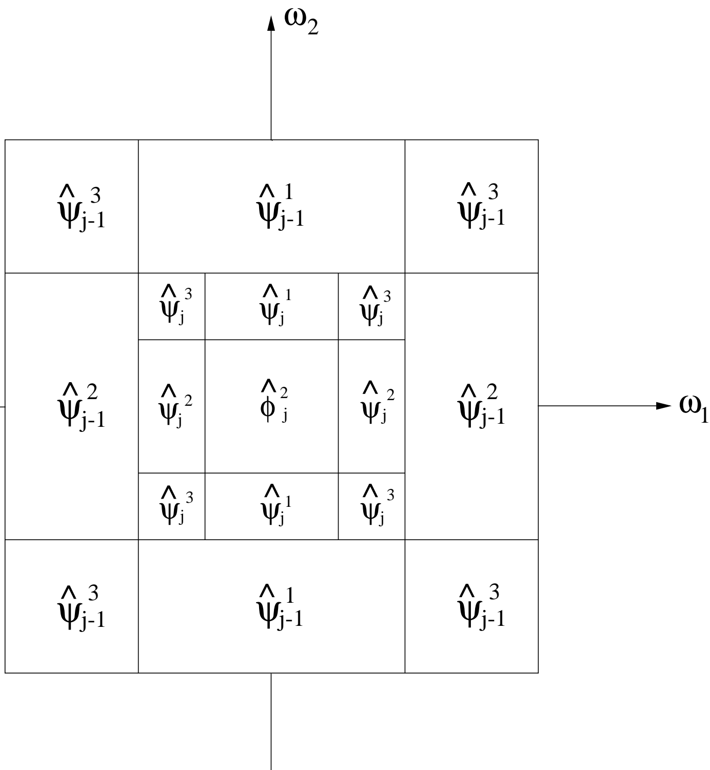
Fig. 7.23. A Wavelet Tour of Signal Processing, 3 rd ed. These dyadic rectangles indicate the regions where the energy of \hat{\psi}_{j,n}^k is mostly concentrated, for 1 \leq k \leq 3 . Image approximations at the scale 2^j are restricted to the lower frequency square.
