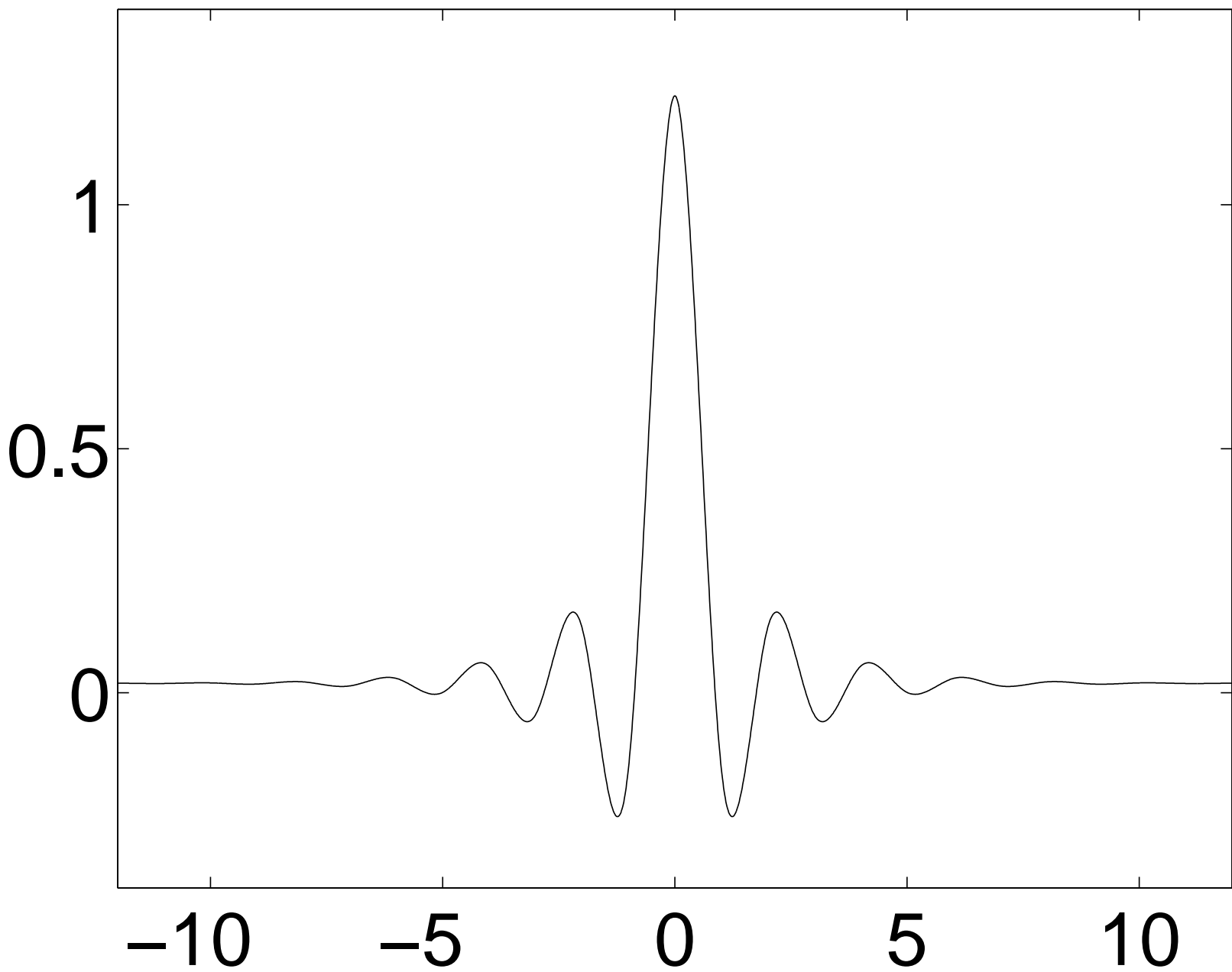
Fig. 7.20. A Wavelet Tour of Signal Processing, 3 rd ed. The dual cubic spline \tilde{\phi}(t) associated to the spline interpolation function \phi(t) .
