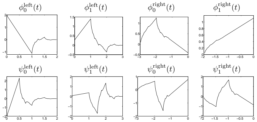
Fig. 7.18. A Wavelet Tour of Signal Processing, 3 rd ed. Boundary scaling functions and wavelets with p = 2 vanishing moments.
