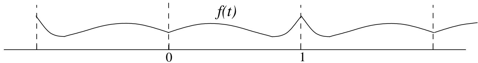
Fig. 7.17. A Wavelet Tour of Signal Processing, 3 rd ed. The folded signal f^{\text{repl}}(t) is 2 periodic, symmetric about t = 0 and t = 1 , and equal to f(t) on [0, 1] .
