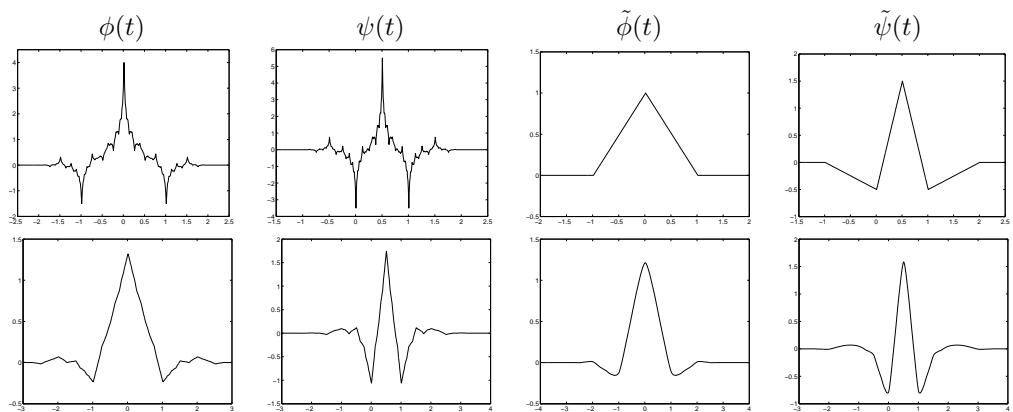
Fig. 7.15. A Wavelet Tour of Signal Processing, 3 rd ed. Biorthogonal wavelets and scaling functions, with p = 2 and \tilde{p} = 2 (top row) and with p = 4 and \tilde{p} = 4 (bottom row).
