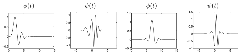
Fig. 7.11. A Wavelet Tour of Signal Processing, 3 rd ed. Daubechies (first two) and Symmlets (last two) scaling functions and wavelets with p = 8 vanishing moments.
