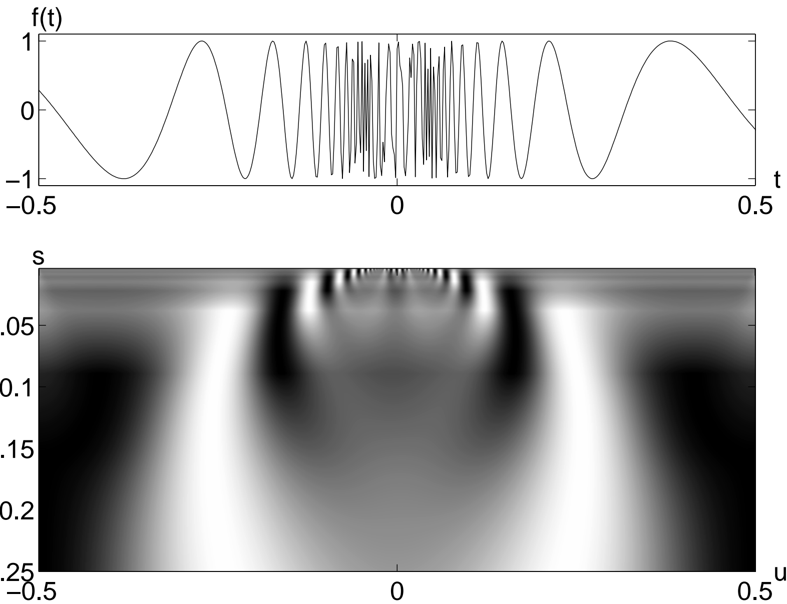
Fig. 6.3. A Wavelet Tour of Signal Processing, 3 rd ed. Wavelet transform of f(t) = \sin(at^{-1}) calculated with \psi = -\theta' where \theta is a Gaussian. High amplitude coefficients are along a parabola outside the cone of influence of t = 0 .
