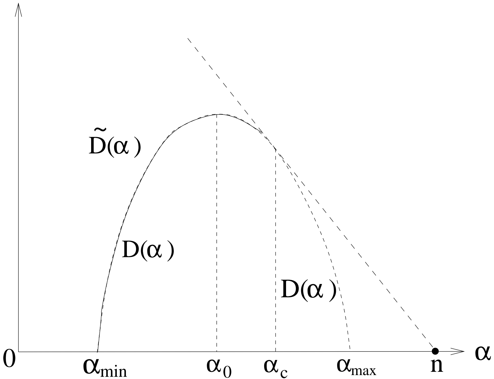
Fig. 6.20. A Wavelet Tour of Signal Processing, 3 rd ed. If \psi has n vanishing moments, in presence of a C^\infty perturbation the computed spectrum \tilde{D}(\alpha) is identical to the true spectrum D(\alpha) for \alpha \leq \alpha_c . Its support is reduced to \{n\} for \alpha > \alpha_c .
