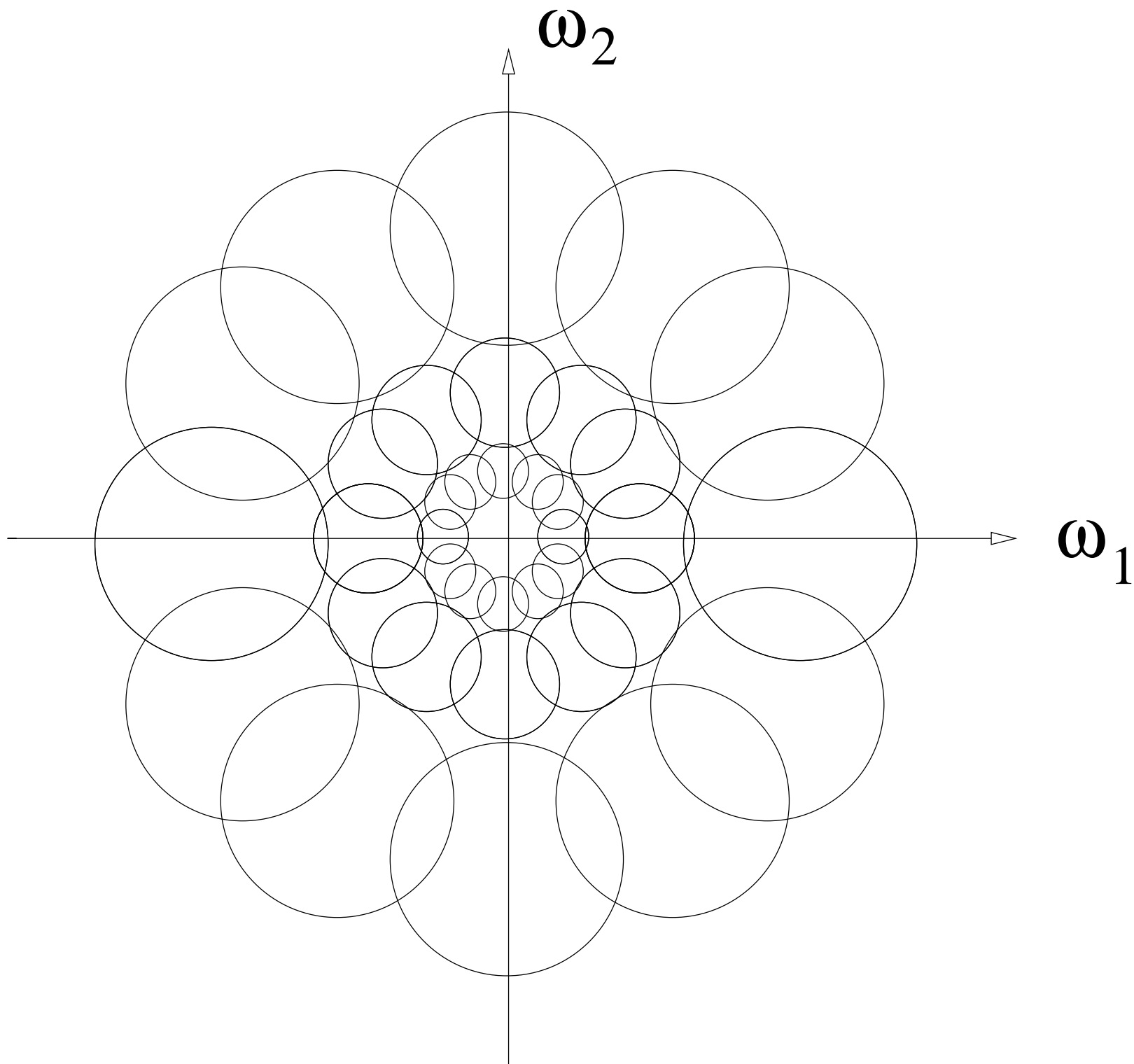
Fig. 5.8. A Wavelet Tour of Signal Processing, 3 rd ed. Each circle represents the frequency domain in a direction \alpha + \pi/2 where the amplitude of a Gabor wavelet Fourier transform |\hat{\psi}_{2^j}^\alpha(\omega)| is large. It is proportional to 2^{-j} and its position rotates with \alpha .
