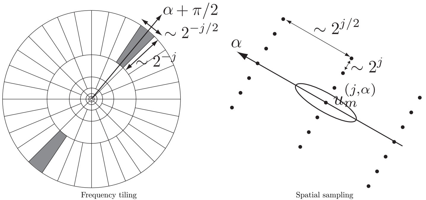
Fig. 5.12. A Wavelet Tour of Signal Processing, 3 rd ed. Left: Curvelet polar tiling of the frequency plane with with parabolic wedges. Right: curvelet sampling grid u_m^{(j,\alpha)} at a scale 2^j and direction \alpha .
