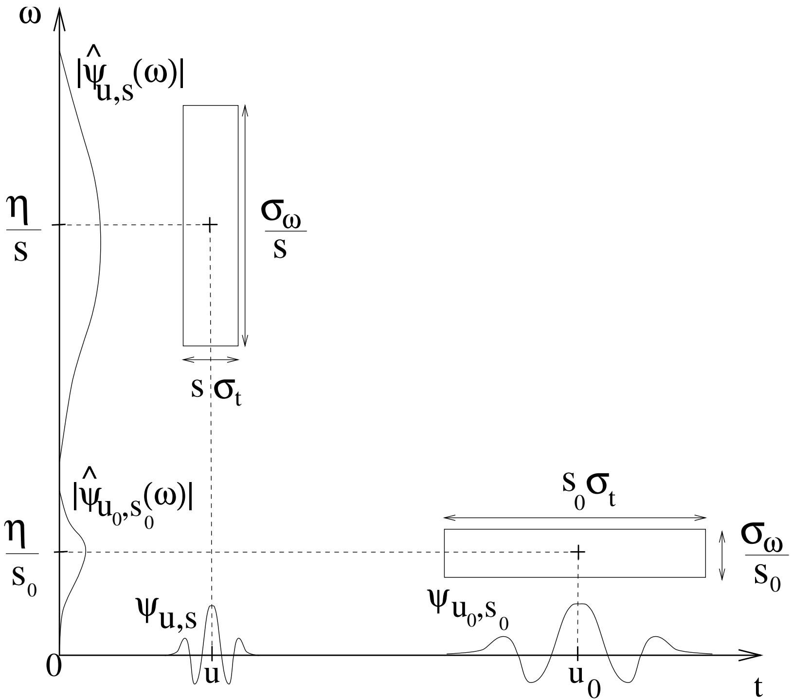
Fig. 4.9. A Wavelet Tour of Signal Processing, 3 rd ed. Heisenberg boxes of two wavelets. Smaller scales decrease the time spread but increase the frequency support, which is shifted towards higher frequencies.
