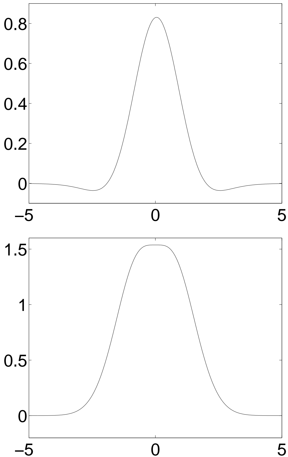
Fig. 4.8. A Wavelet Tour of Signal Processing, 3 rd ed. Scaling function associated to a Mexican hat wavelet and its Fourier transform.
