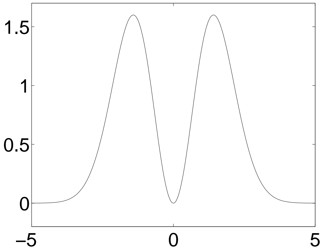
Fig. 4.6. A Wavelet Tour of Signal Processing, 3 rd ed. Mexican hat wavelet for \sigma = 1 and its Fourier transform.
