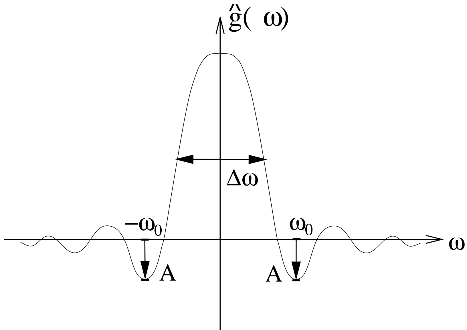
Fig. 4.4. A Wavelet Tour of Signal Processing, 3 rd ed. The energy spread of \hat{g} is measured by its bandwidth \Delta\omega and the maximum amplitude A of the first side-lobes, located at \omega = \pm\omega_0 .
