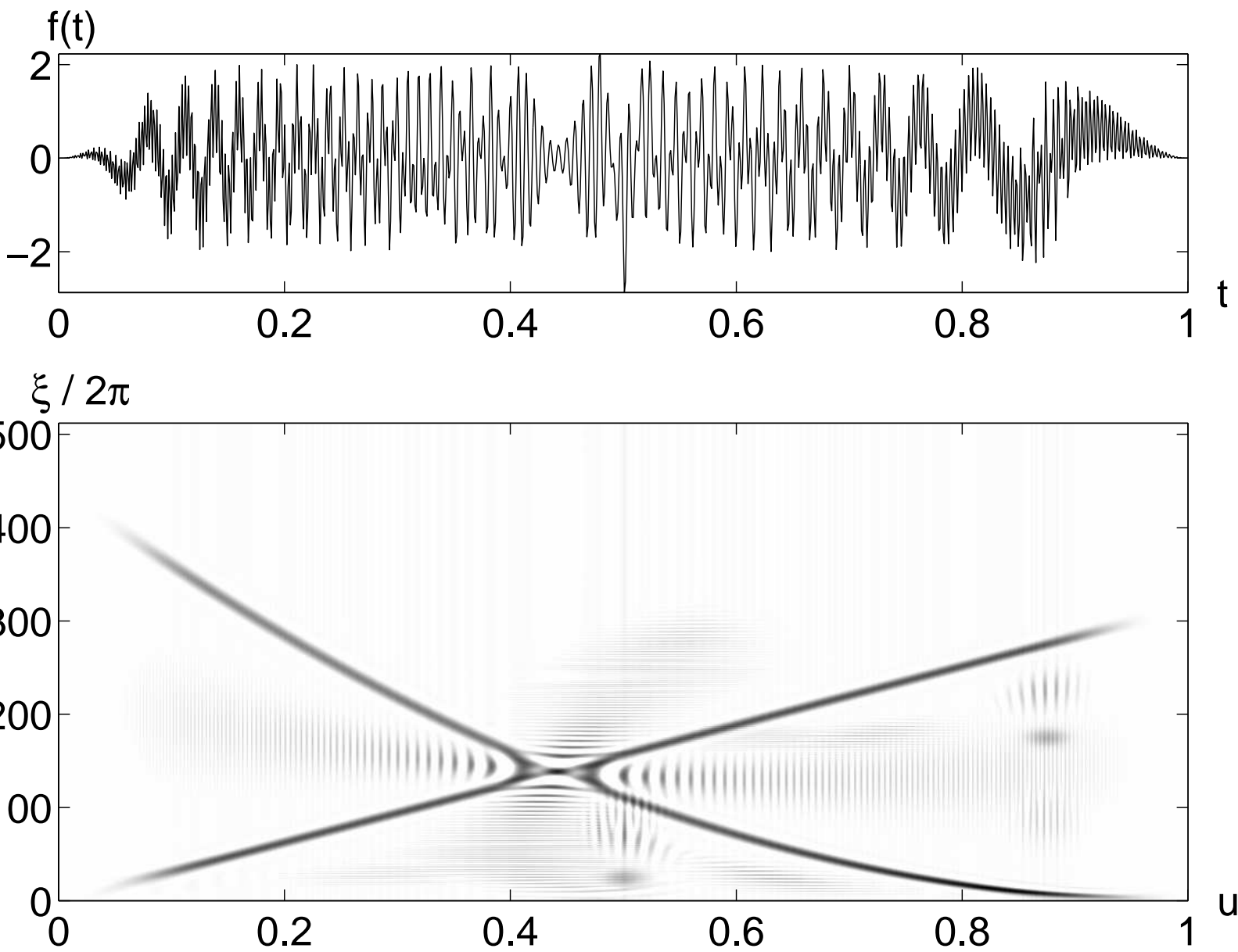
Fig. 4.21. A Wavelet Tour of Signal Processing, 3 rd ed. Choi-William distribution P_K f_a(u, \xi) of the analytic part of the signal shown at the top. The interferences remain visible.
