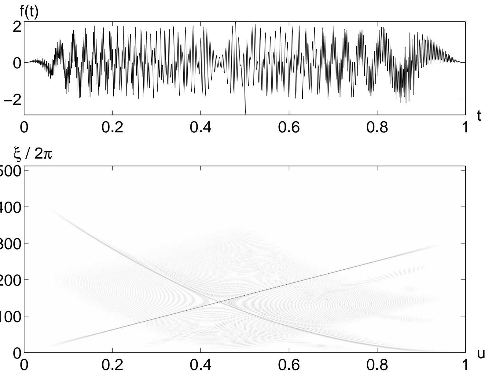
Fig. 4.19. A Wavelet Tour of Signal Processing, 3 rd ed. The bottom displays the Wigner-Ville distribution P_V f_a(u, \xi) of the analytic part of the top signal.
