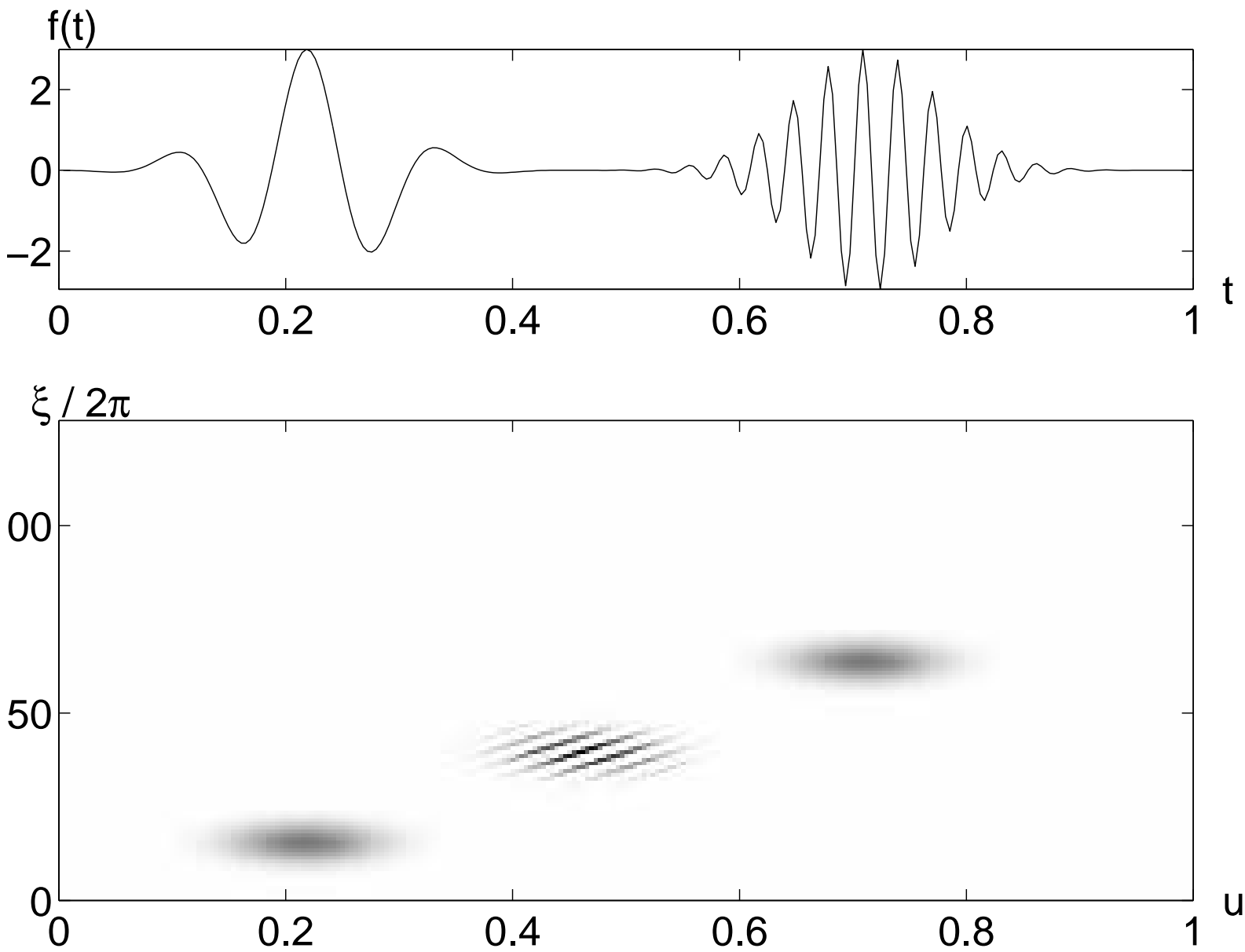
Fig. 4.18. A Wavelet Tour of Signal Processing, 3 rd ed. Wigner-Ville distribution P_V f(u, \xi) of two Gabor atoms shown at the top. The oscillating interferences are centered at the middle time-frequency location.
