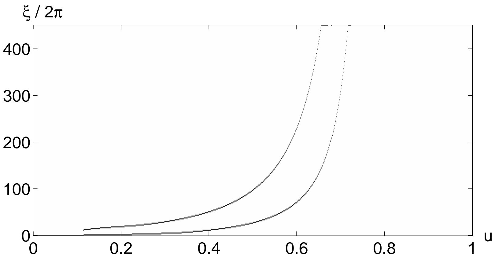
Fig. 4.17. A Wavelet Tour of Signal Processing, 3 rd ed. (a): Normalized scalogram \eta^{-1}\xi P_W f(u, \xi) of two hyperbolic chirps. (b): Wavelet ridges.
