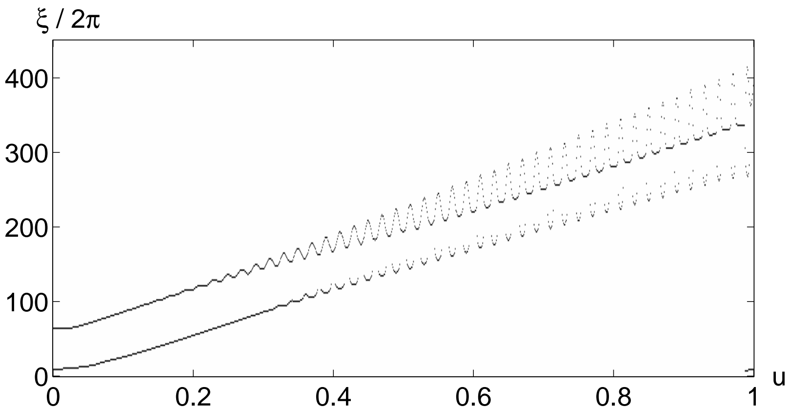
Fig. 4.16. A Wavelet Tour of Signal Processing, 3 rd ed. (a): Normalized scalogram \eta^{-1}\xi P_W f(u, \xi) of two parallel linear chirps. (b): Wavelet ridges.
