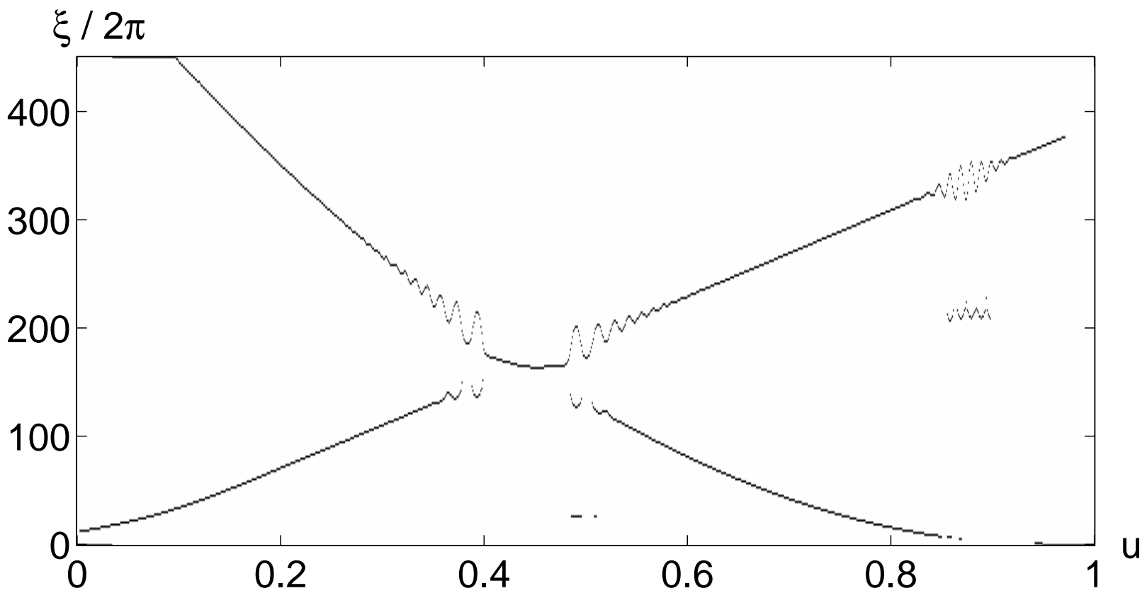
Fig. 4.15. A Wavelet Tour of Signal Processing, 3 rd ed. Ridge support calculated from the scalogram.
