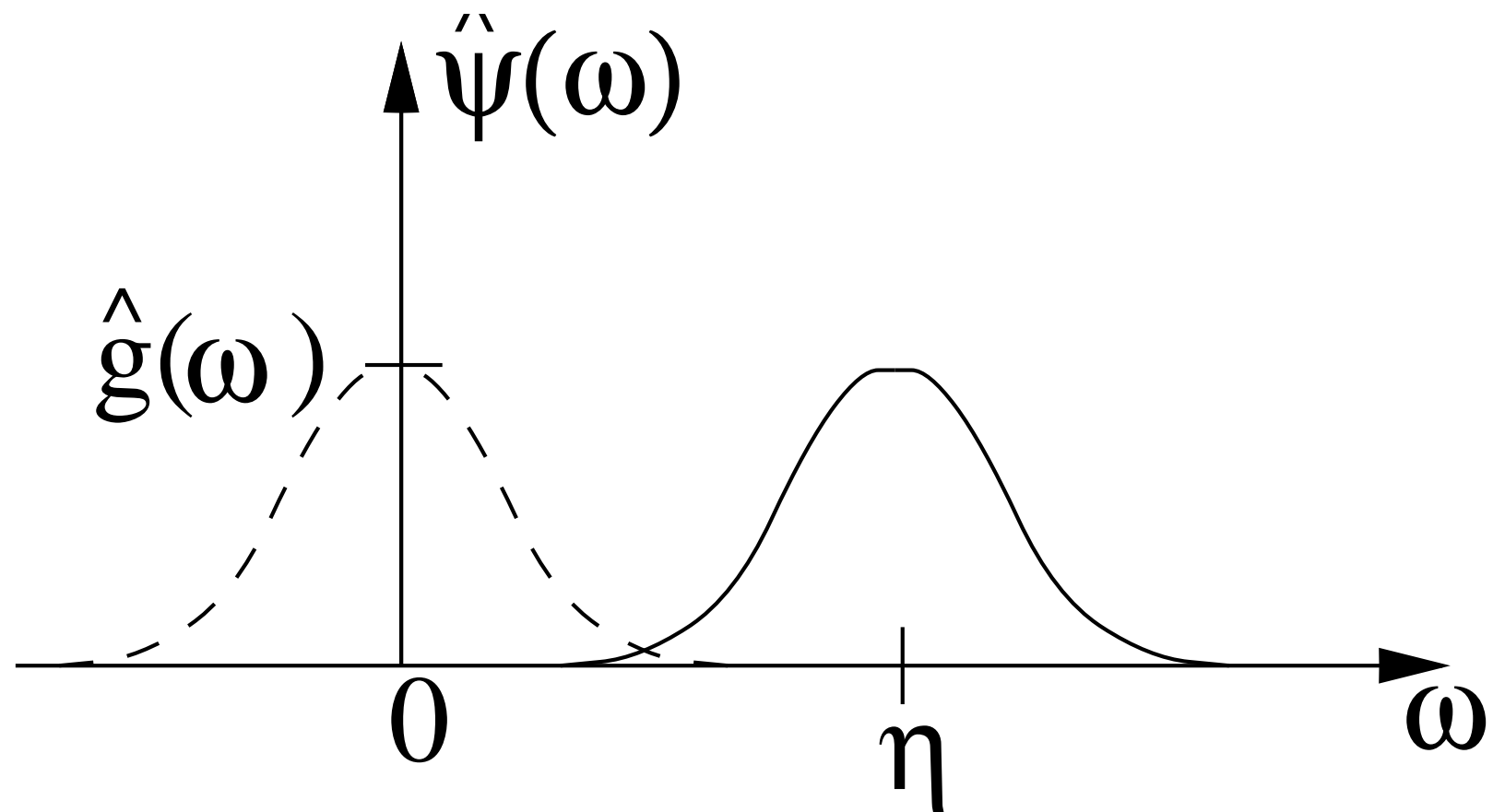
Fig. 4.10. A Wavelet Tour of Signal Processing, 3 rd ed. Fourier transform \hat{\psi}(\omega) of a wavelet \psi(t) = g(t) \exp(i\eta t) .
