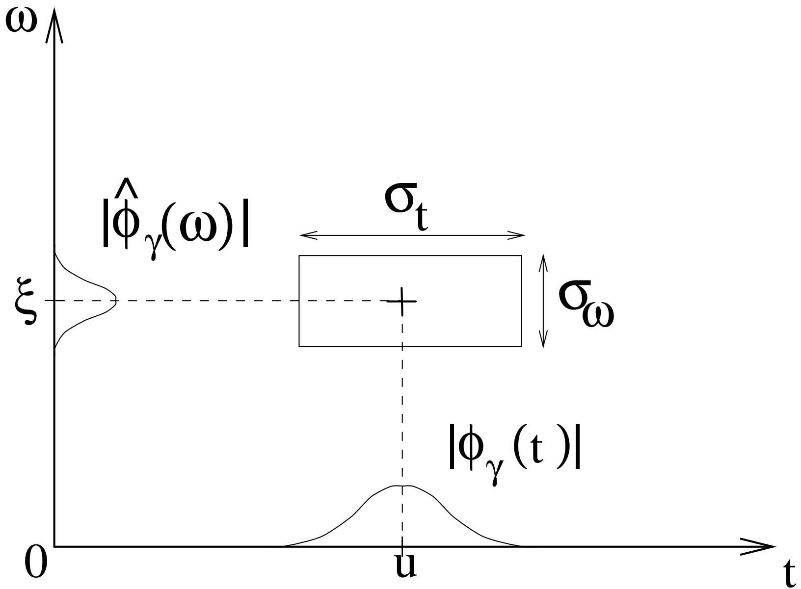
Fig. 4.1. A Wavelet Tour of Signal Processing, 3 rd ed. Heisenberg box representing an atom \phi_\gamma .
